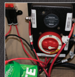
DUAL BATTERY HARNESS W/SWITCH
